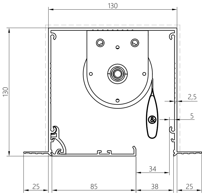
HEAD BOX S130x130SS
