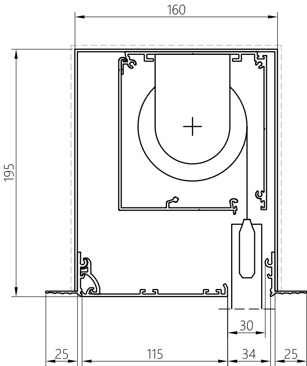
SIDE BOX C160x75SS (OPTIONAL)
