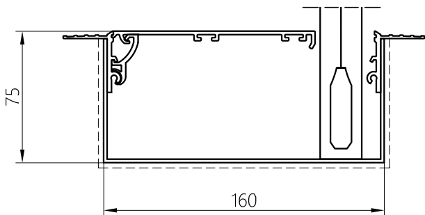
HEM BAR BOX C160x75SS (OPTIONAL)
