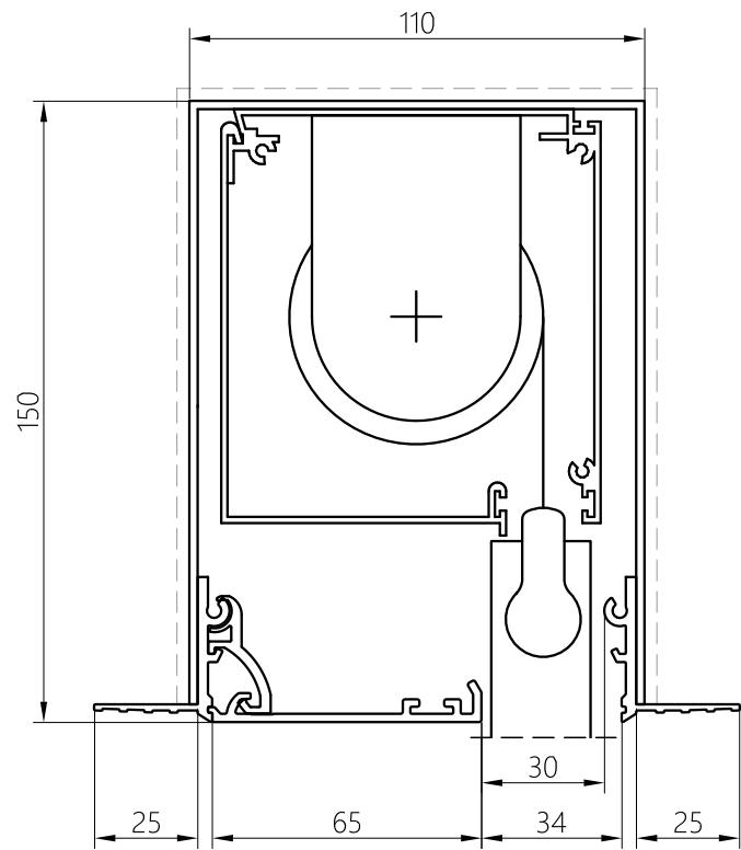
SIDE BOX C110x50SS (OPTIONAL)
