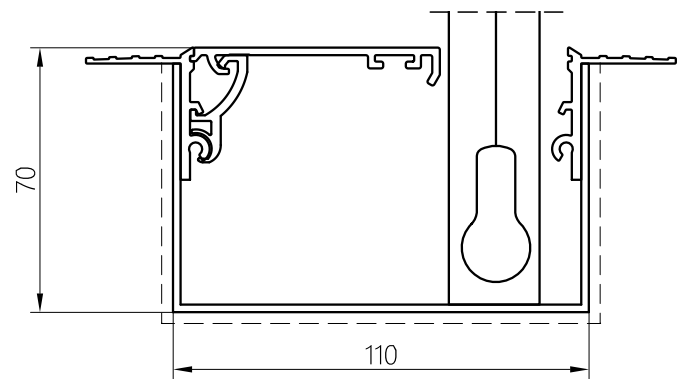
HEM BAR BOX C110x70SS (OPTIONAL)
