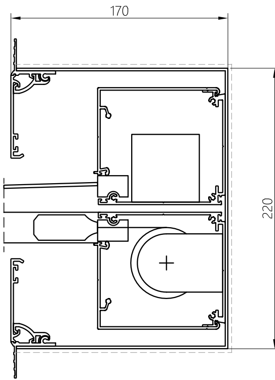
HEM BAR BOX C220x170SS (OPTIONAL)
