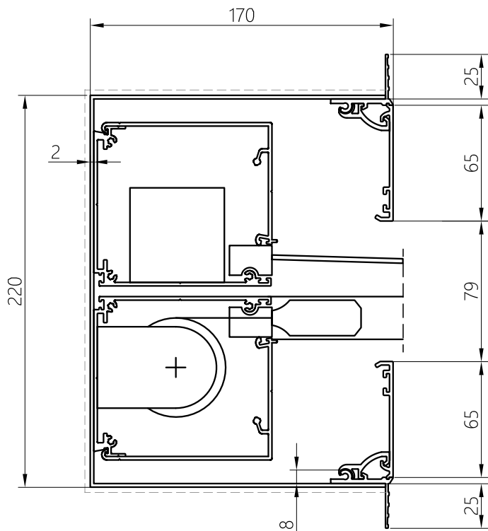
HEAD BOX C220x170SS
