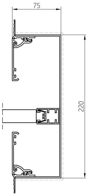
SIDE BOX C220x75SS (OPTIONAL)
